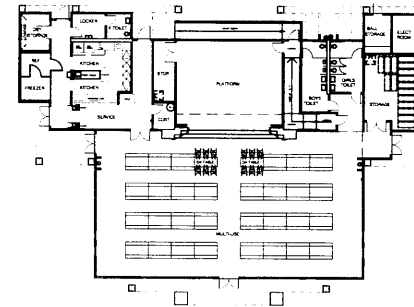
MULTI-USE/KITCHEN FLOOR PLAN
