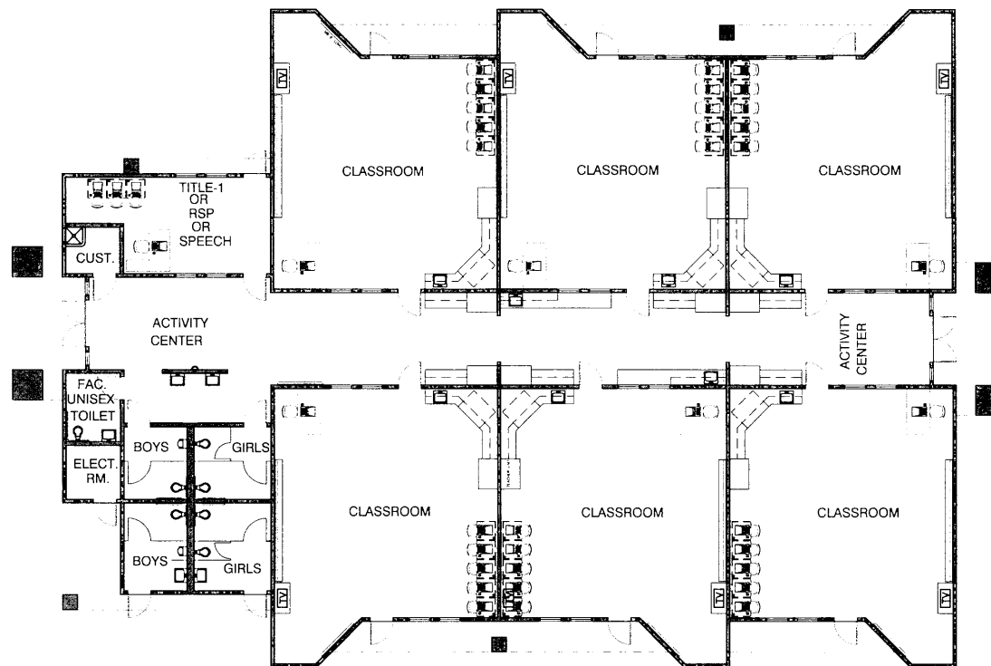
CLASSROOM FLOOR PLAN BUILDINGS "D", "E", "F" & "G".
