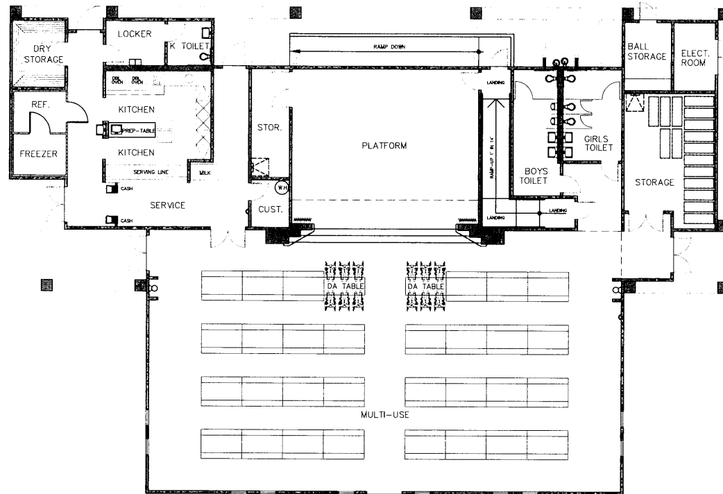
MULTI-USE/KITCHEN FLOOR PLAN
