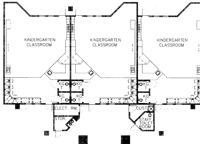
KINDERGARTEN FLOOR PLAN BUILDING 'B'
