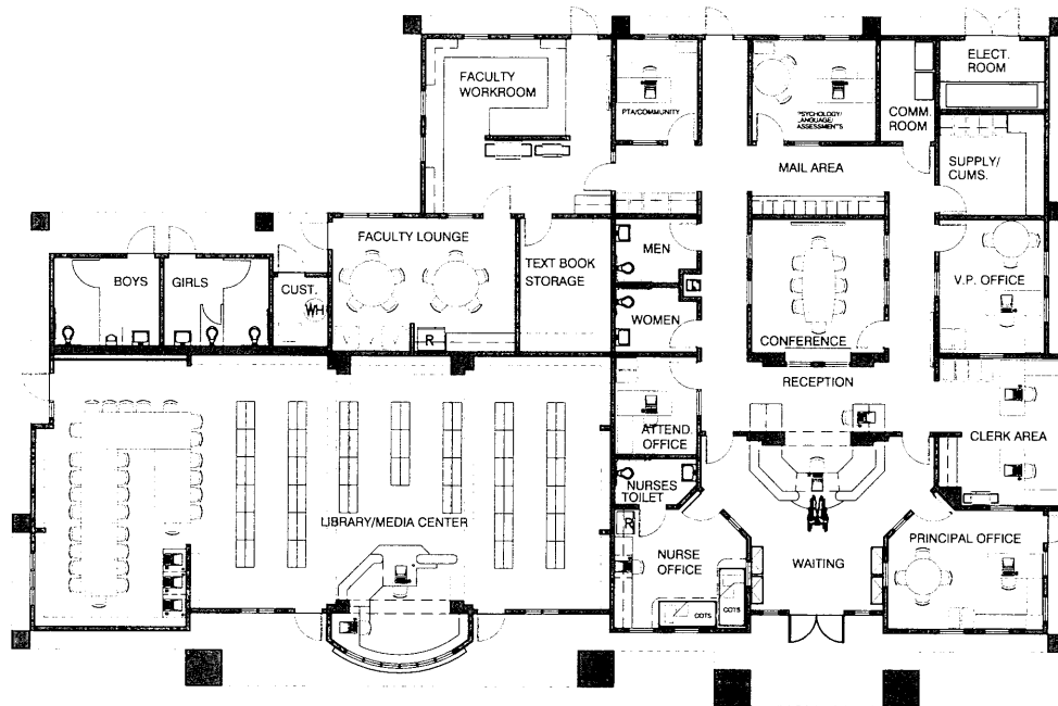
ADMIN./LIBRARY/MEDIA CENTER FLOOR PLAN BUILDING 'A'
