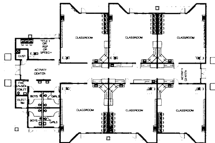
CLASSROOM FLOOR PLAN
