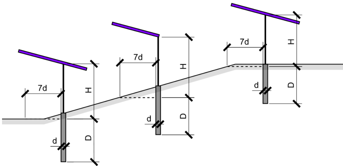
Figure 5.8: Sloped Sites
