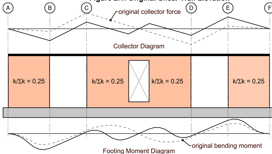
Figure 2.2: Shear Wall Elevation after Alteration
