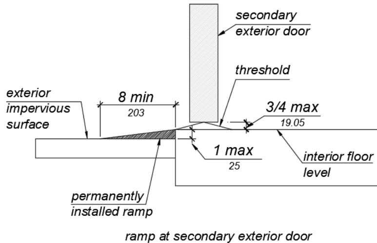
FIGURE 11B-809.8 (d) RAMP AT SECONDARY EXTERIOR DOOR.
