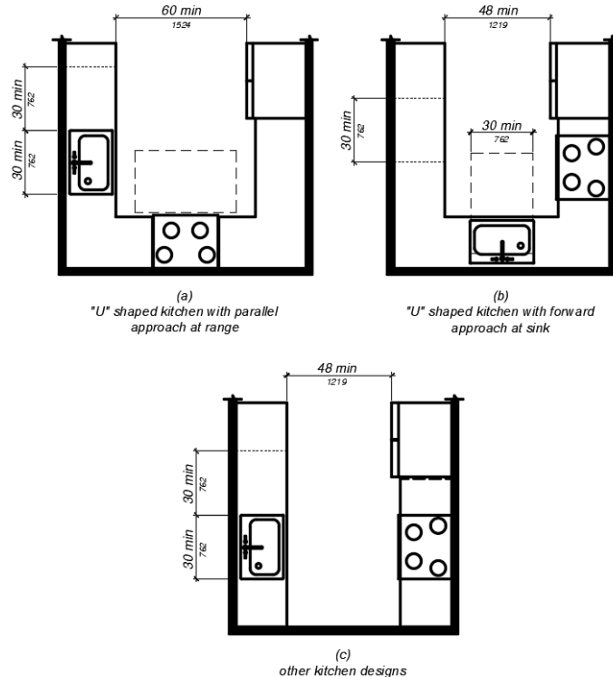
FIGURE 11B-809.9.2 CLEAR WIDTH AT KITCHENS.
