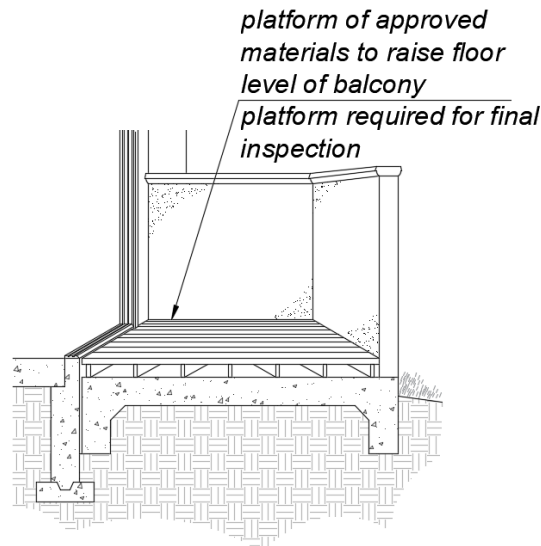
FIGURE 11B-809.8 (c) PLATFORM AT SECONDARY EXTERIOR DOOR.
