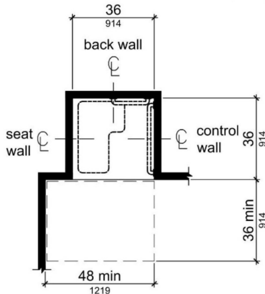
FIGURE 11B.809.10.6.3 TRANSFER TYPE SHOWER CLEARANCE
