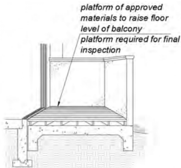
FIGURE 11B-809.8.3.1 (3) PLATFORM AT SECONDARY EXTERIOR DOOR
