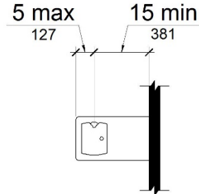
Figure 11B-602.5 Drinking Fountain Spout Location
