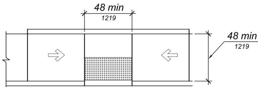
Figure 11B-406.3.2 Parallel Curb Ramps
