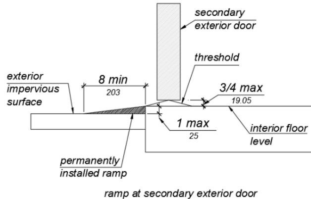
FIGURE 11B-809.8.3.1 (4) RAMP AT SECONDARY EXTERIOR DOOR
