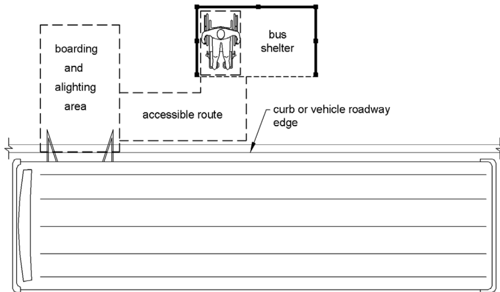
Figure 11B-810.3 Bus Shelters
