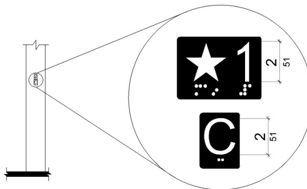
Figure 11B-411.2.3 Floor Designation and Car Designation Signs on Jambs of Destination-Oriented Elevator Hoistway (begin strike-out) Signs (end strike-out) (begin underline) Entrances (end underline)
