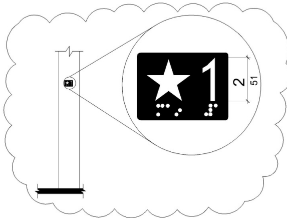
Figure 11B-407.2.3.1 Floor Designations on Jamb of Elevator Hoistway Entrance Entrances
