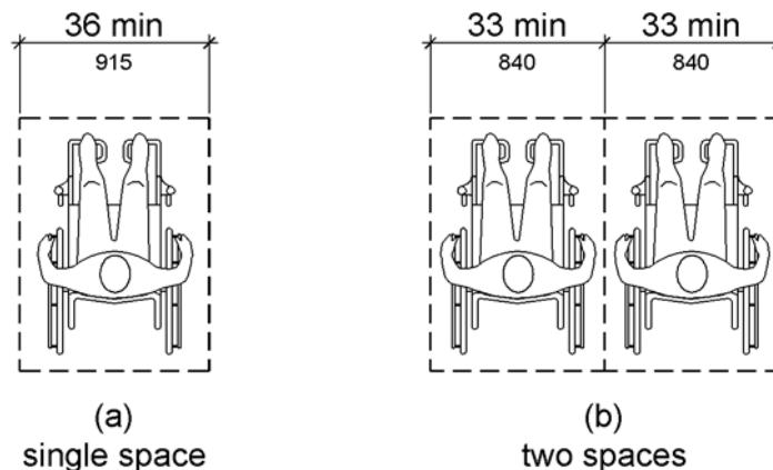
Figure 11B-802.1.2 Width of Wheelchair Spaces in Assembly Areas
