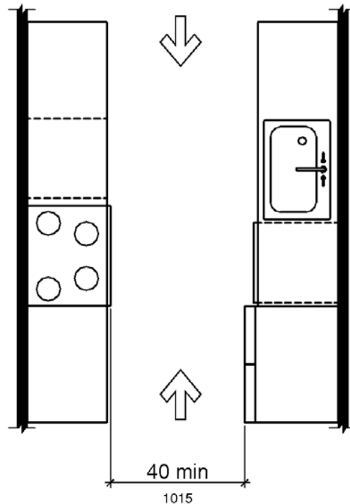
Figure 11B-804.2.1 Pass Through Kitchens
