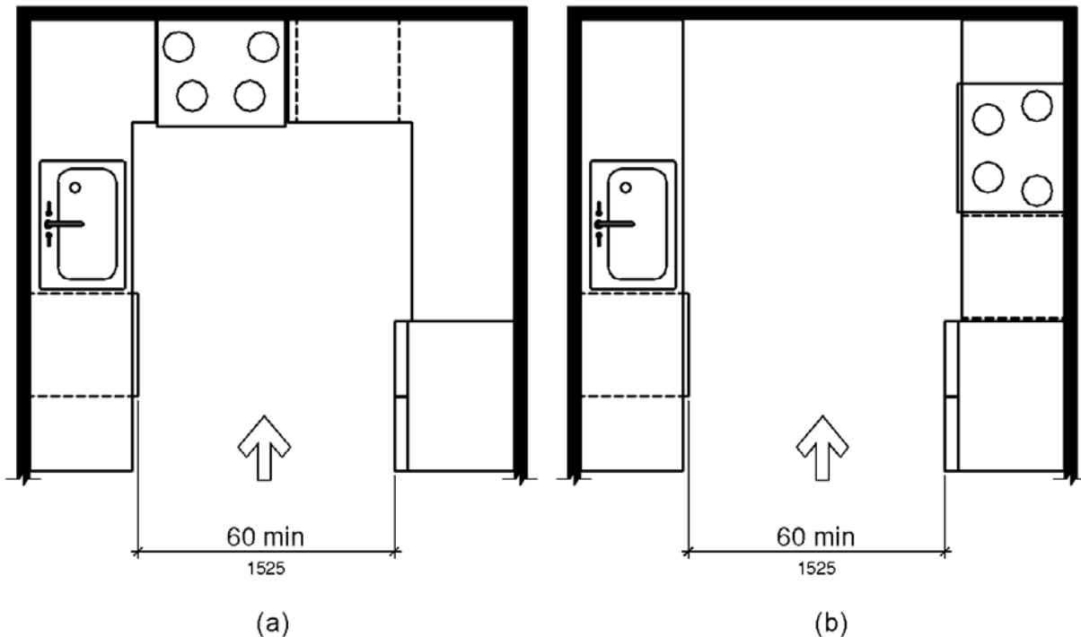
Figure 11B-804.2.2 U-Shaped Kitchens
