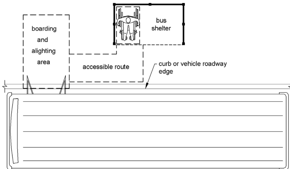
Figure 11B-810.3 Bus Shelters
