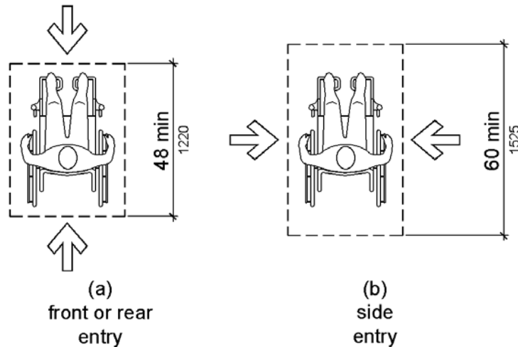
Figure 11B-802.1.3 Depth of Wheelchair Spaces in Assembly Areas
